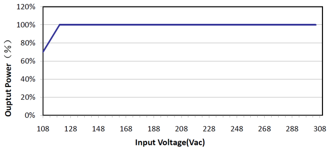
© P_O / P_{MAX} vs. INPUT VOLTAGE CURVE
