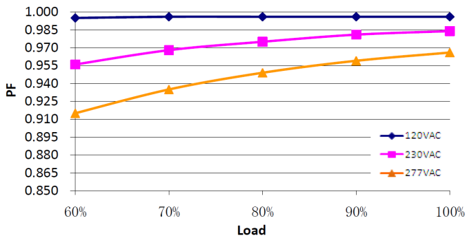
© POWER FACTOR vs. LOAD CURVE
