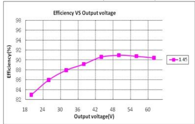
GLUP-120X062Z ( Vin=277Vac )
