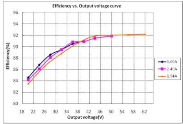
GLUP-120X170Z ( Vin=230Vac )
