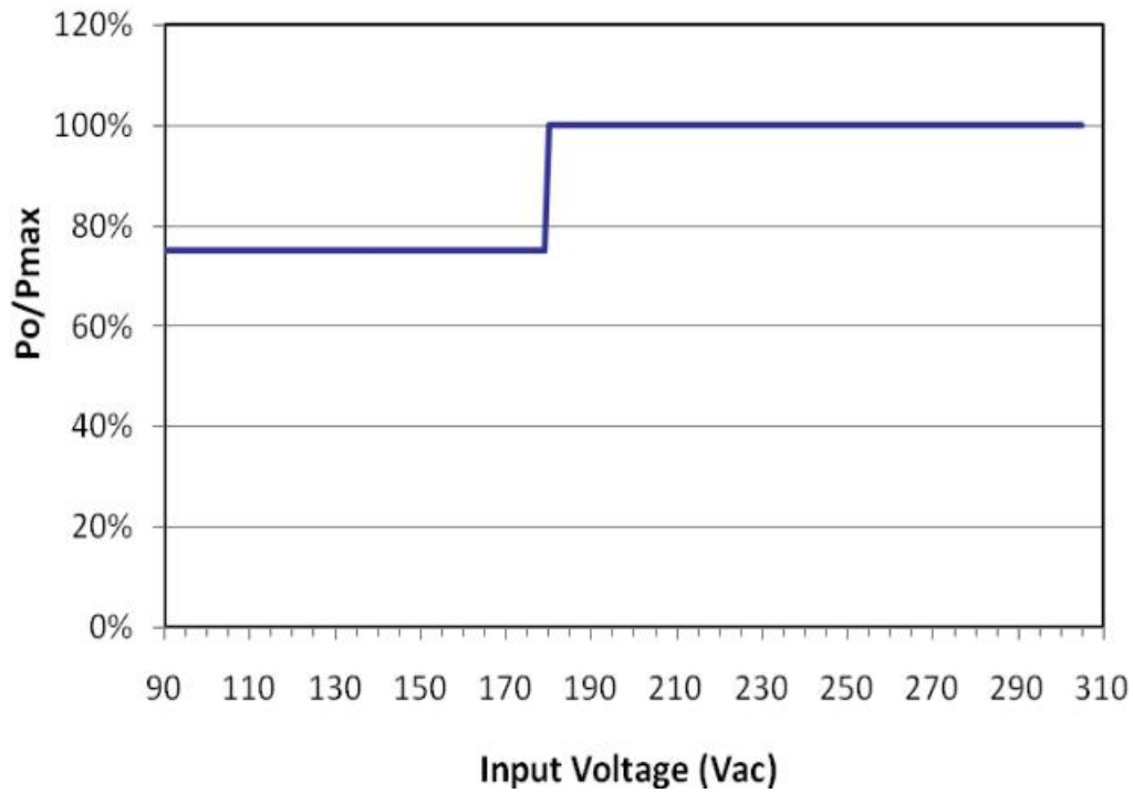
Po/Pmax vs. Input Voltage Curve
