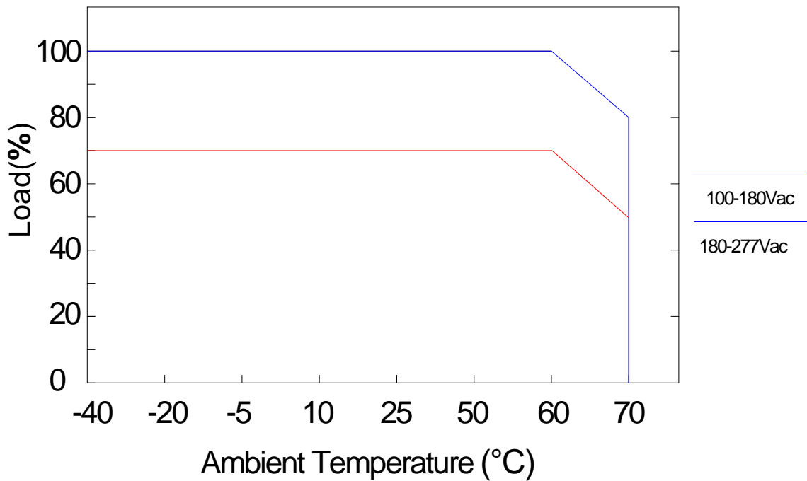
Derating Curve
