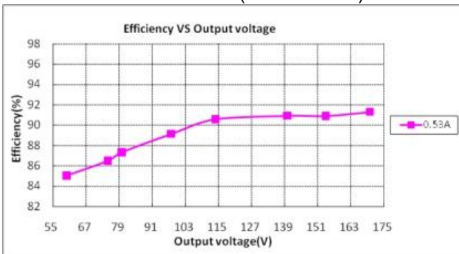
GLUP-120X170Z ( Vin=115Vac )
