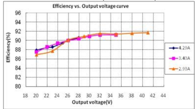
GLUP-120X041Z ( Vin=230Vac )
