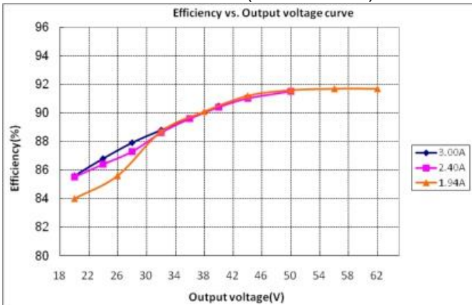
GLUP-120X170Z ( Vin=115Vac )
