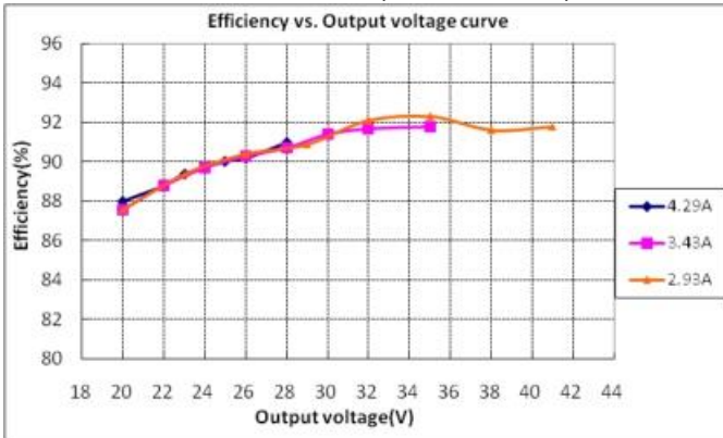
GLUP-120X062Z ( Vin=230Vac )
