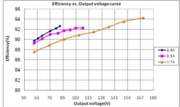
GLUP-120X170Z ( Vin=230Vac )
