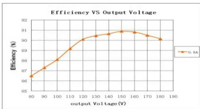
GLCP-240X180Z (Vin=115Vac)
