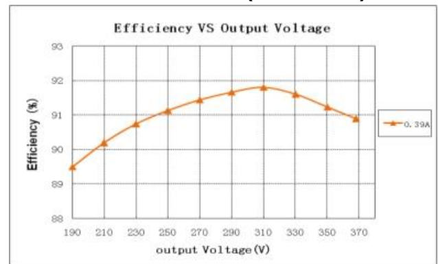
GLCP-240X368Z (Vin=115Vac)
