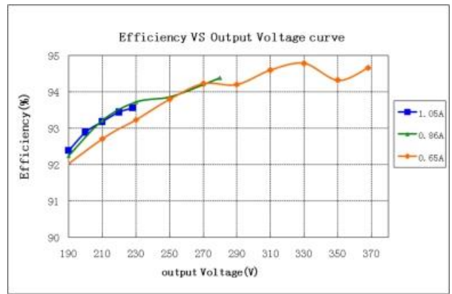
GLCP-240X368Z (Vin=277Vac)
