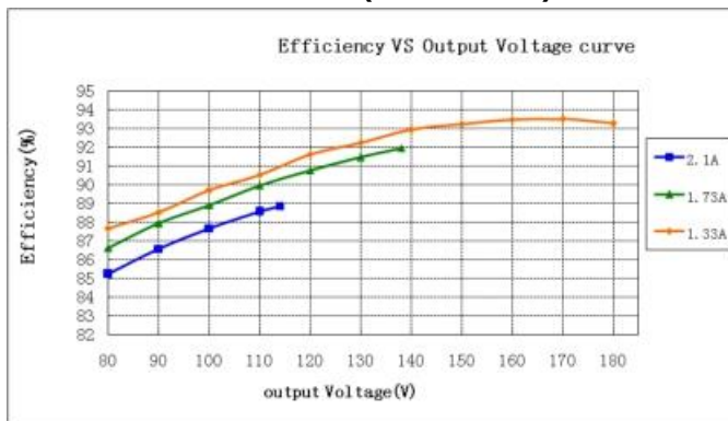
GLCP-240X180Z (Vin=277Vac)
