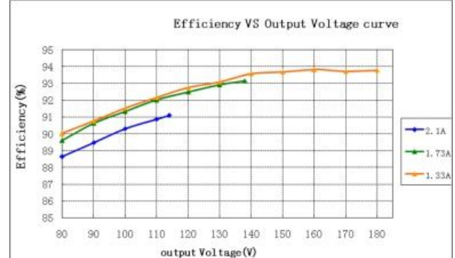
GLCP-240X180Z (Vin=230Vac)
