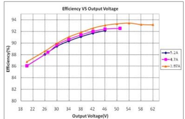
GLCP-240X180Z (Vin=230Vac)
