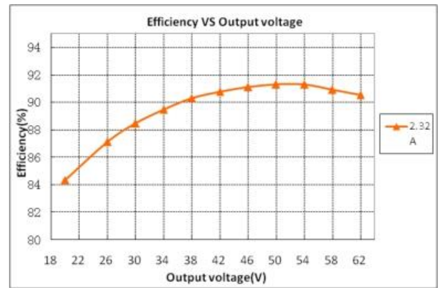
GLCP-240X062Z (Vin=277Vac)
