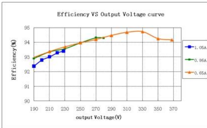
GLCP-240X368Z (Vin=230Vac)
