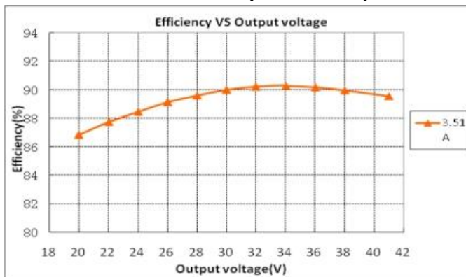
GLCP-240X041Z (Vin=115Vac)
