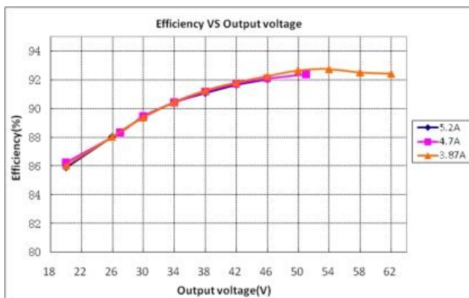
GLCP-240X180Z (Vin=115Vac)
