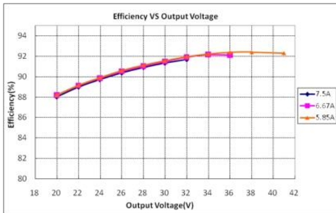
GLCP-240X062Z (Vin=230Vac)
