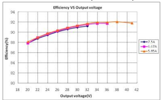
GLCP-240X041Z (Vin=230Vac)
