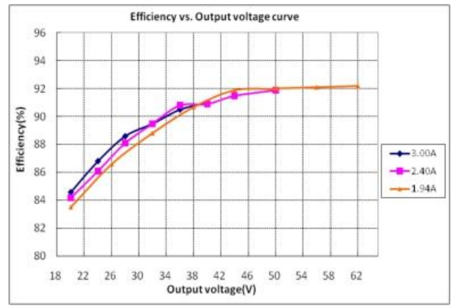
GLCP-120X170Z ( Vin=230Vac )
