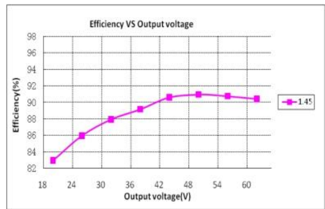
GLCP-120X062Z ( Vin=277Vac )
