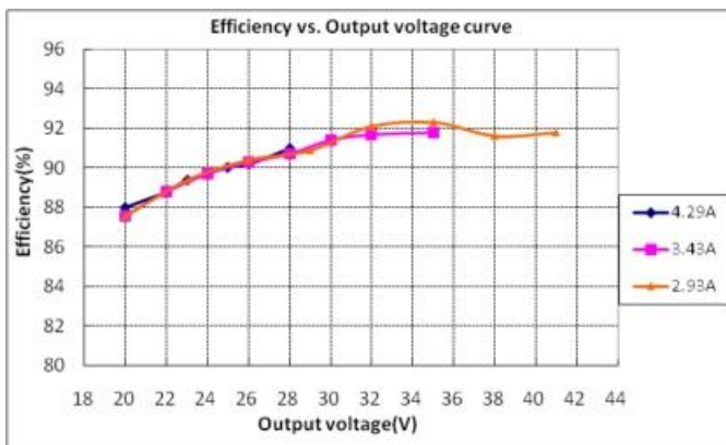
GLCP-120X062Z ( Vin=230Vac )
