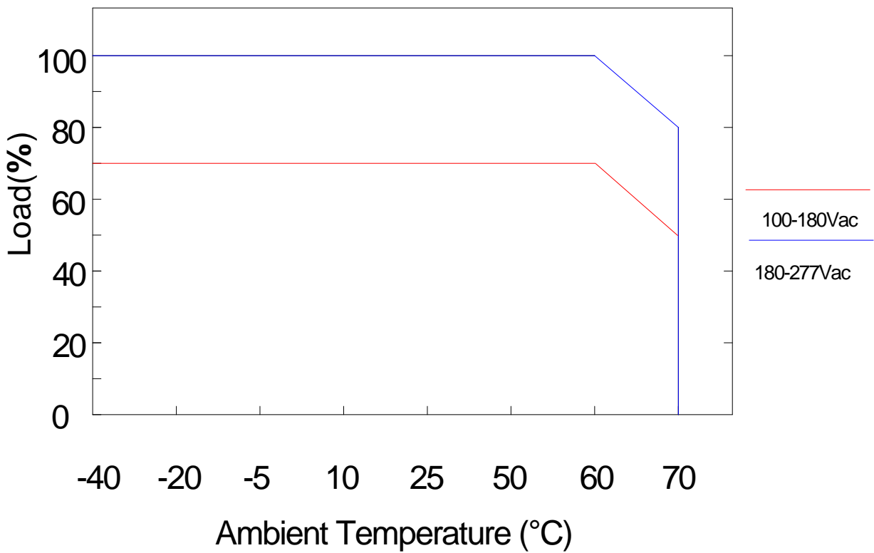
Derating Curve
