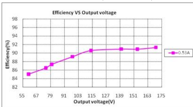
GLCP-120X170Z ( Vin=115Vac )
