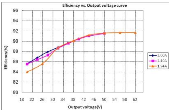
GLCP-120X170Z ( Vin=115Vac )
