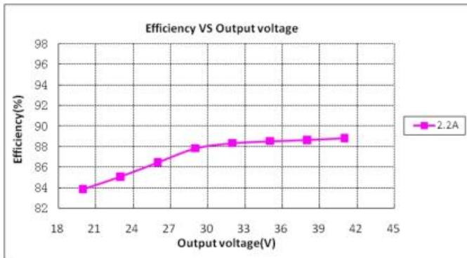
GLCP-120X041Z ( Vin=277Vac )
