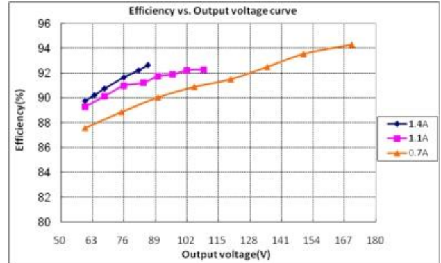
GLCP-120X170Z ( Vin=230Vac )
