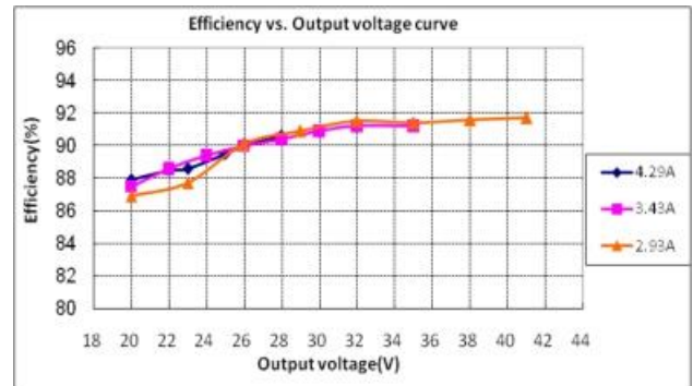
GLCP-120X041Z ( Vin=230Vac )
